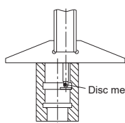
Measuring insert Ø 4 mm
