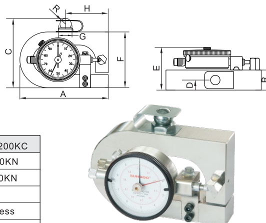
SG Series Analog Force Gauge
