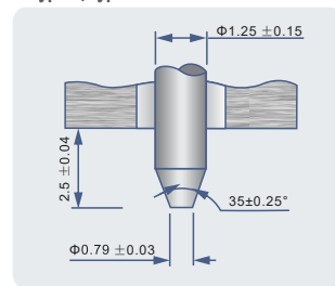
Type A, Type C
