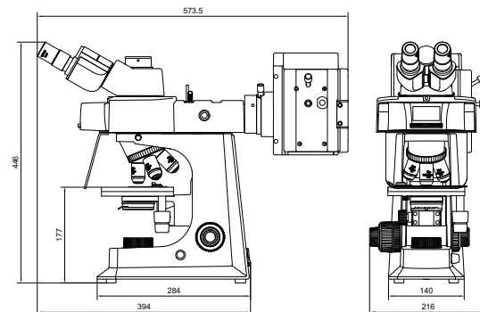
AE-S Fluorescence Microscope Size(mm)
