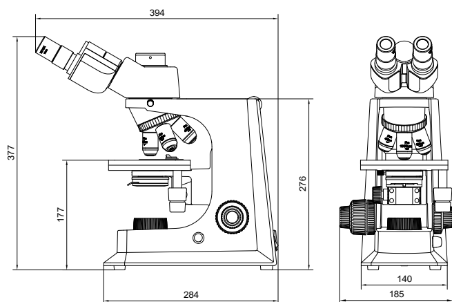
AE-S Series Biological Microscope Size(mm)
