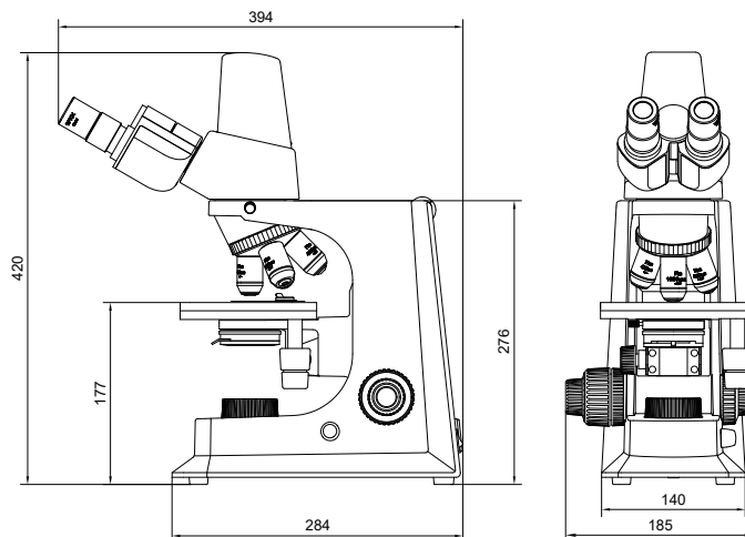
AE-S Fluorescence Microscope Size(mm)
